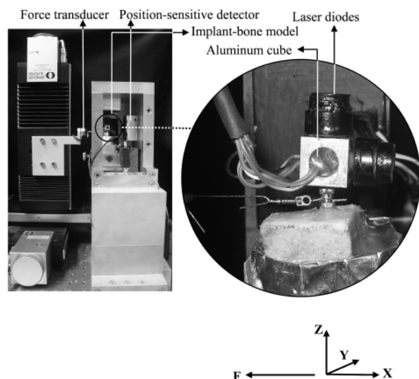
Figure 3 Preparation mounted in the optomechanical system. Force application was applied via a nickel–titanium closed coil spring.
