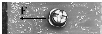
Figure 2 Mini-implant inserted in a bovine bone segment. The force axis was parallel to the bone surface and perpendicular to the long axis of the animal rib.
